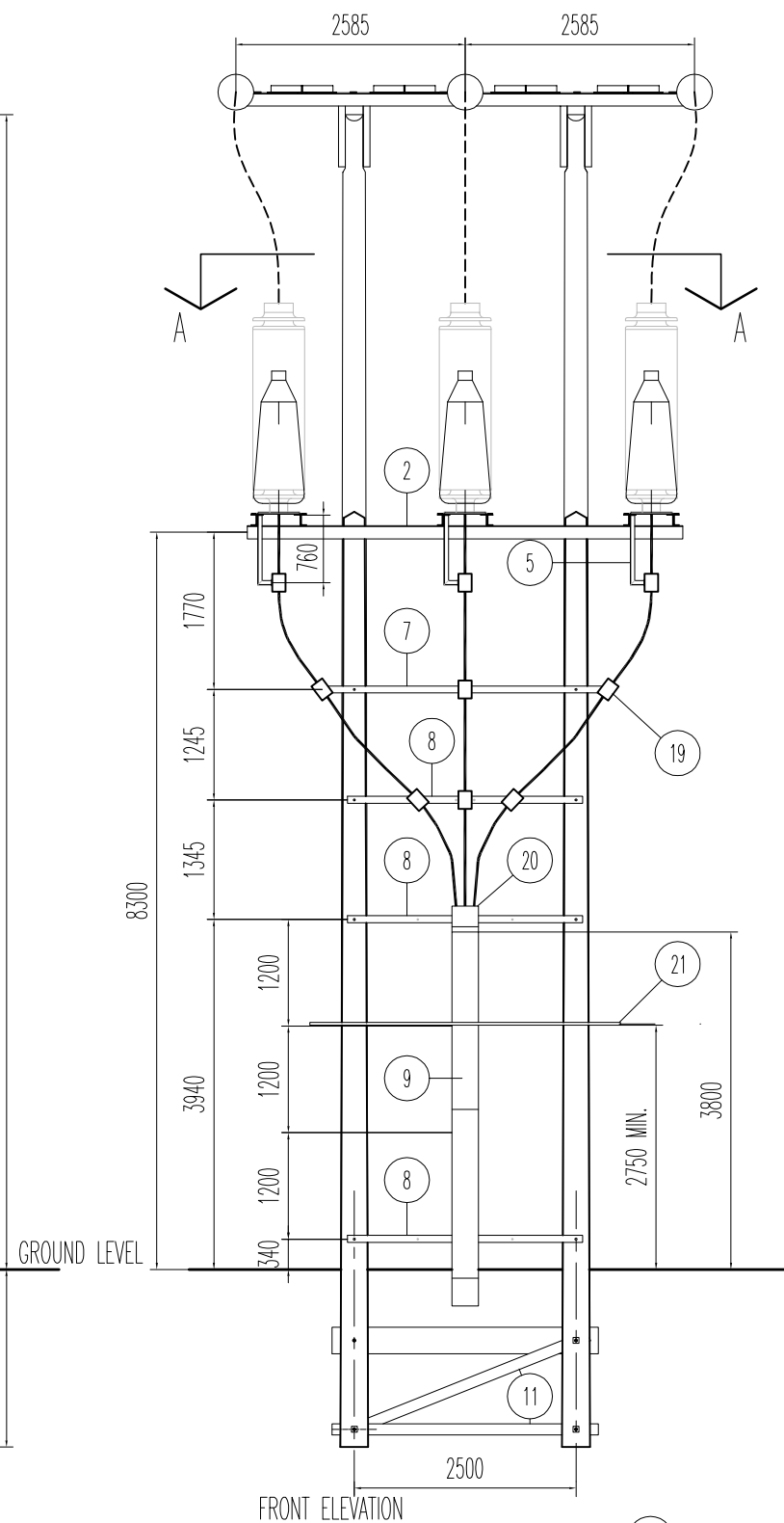
PART DETAIL OF FRONT ELEVATION
